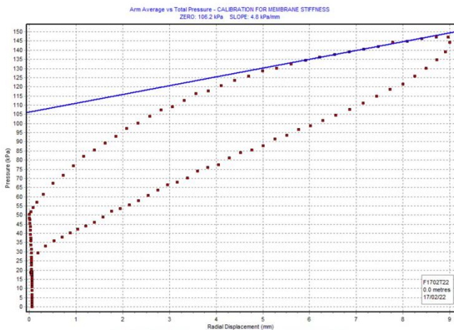
Figure 2.0. HPD membrane stiffness calibration, determining membrane slope.
