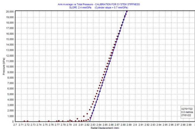
Figure 4.0. HPD system stiffness calibration, determining the entire systems deformation under stress.
