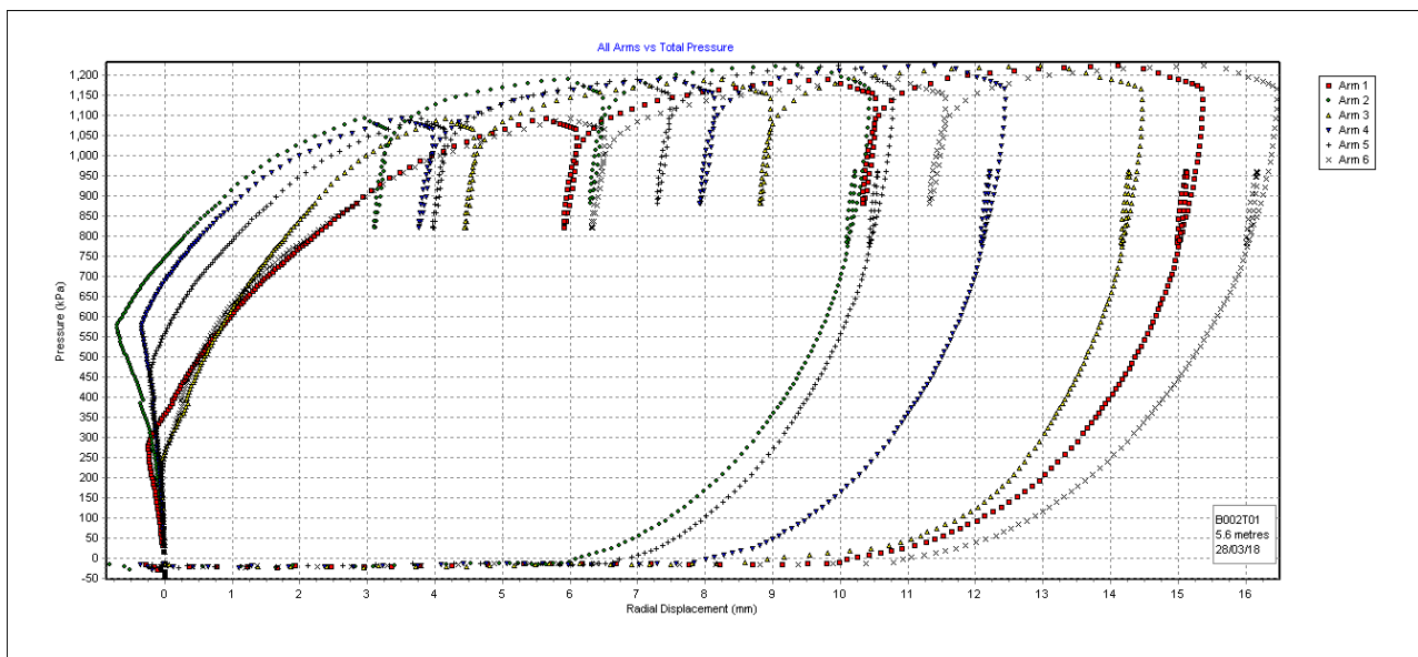
Figure 5.0. Data points as seen on software 'Winlog' during live testing. This plot illustrates the displacement data from all six individual arms (x) versus the total pressure in the probe (y).
