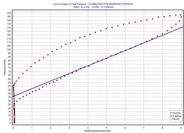
Figure 3.0. HPD membrane stiffness calibration, determining membrane zero.
