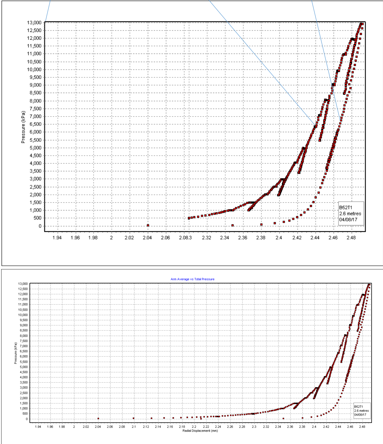
Figure 7.0. Top : blown up/zoomed in test data points and axis. Bottom : The original image of the test in a weak rock. Note the relatively small radial displacement and large total pressure.
